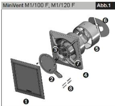
Рис. 1 MiniVent M1/100 F и M1/120 F
