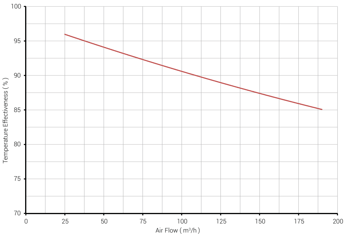
Temperature Effectiveness Graph
