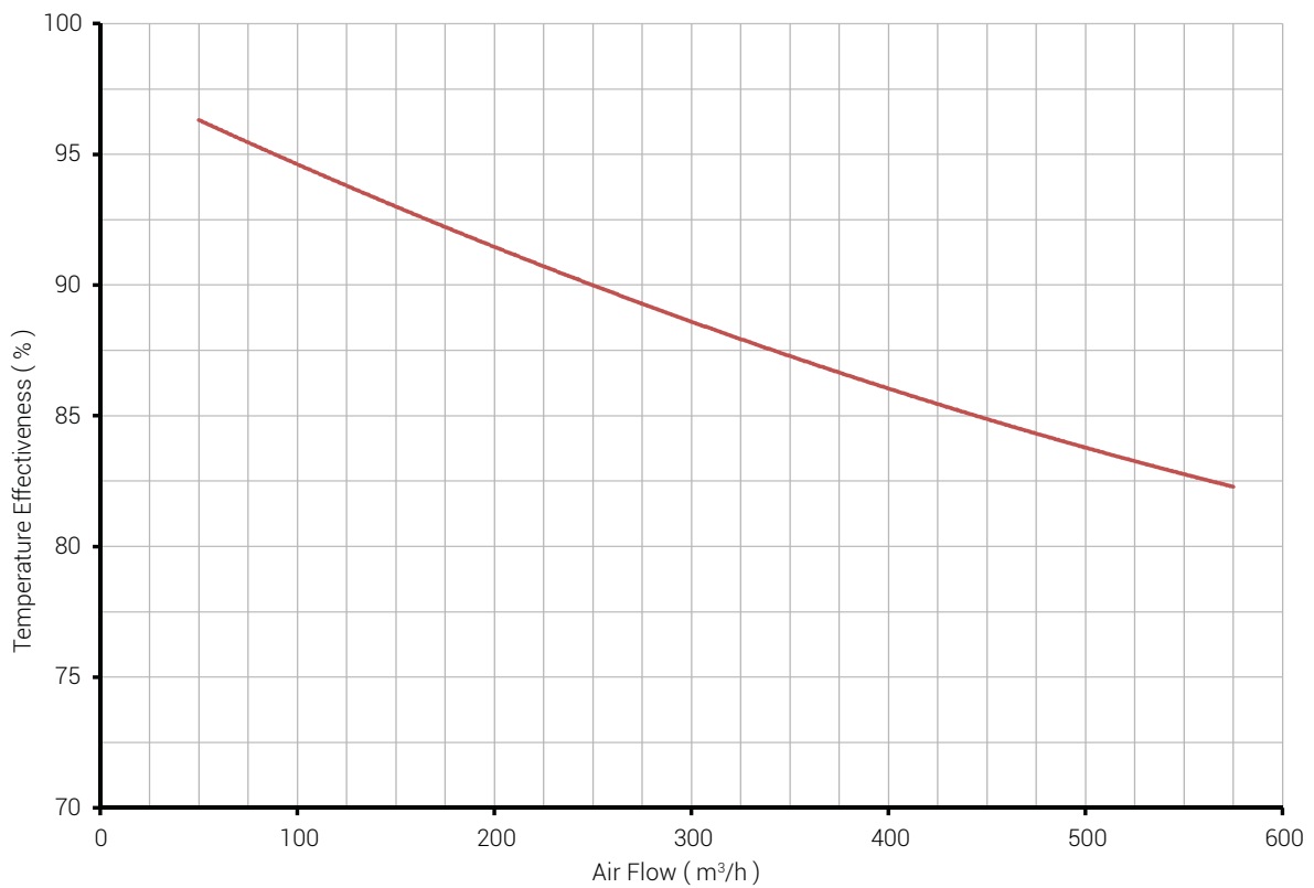
Temperature Effectiveness Graph
